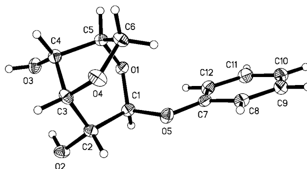
Figure 2. ORTEP diagram of phenyl 3,6-anhydro- \beta -D-glucopyranoside ( C_{12}H_{14}O_5 ). Selected bond lengths [Å] and angles [°]: O(1)–C(5), 1.444(2); O(1)–C(1), 1.401(2); C(2)–C(3), 1.527(3); C(3)–C(4), 1.518(2); O(3)–C(4), 1.407(2); O(2)–C(2), 1.420(2); O(3)–C(4)–C(3), 116.14(14); O(2)–C(2)–C(3), 111.51(15); O(1)–C(1)–O(5), 115.4(14); O(5)–C(1)–C(2), 105.42(12); C(3)–O(4)–C(6), 107.48(12); O(4)–C(6)–C(5), 105.16(13); C(4)–C(5)–C(6), 100.49(13).
